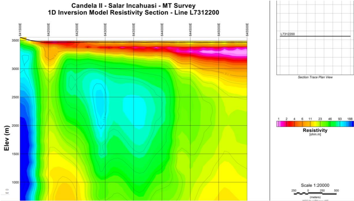
MT Survey line L7312200 down 3850-500masl
