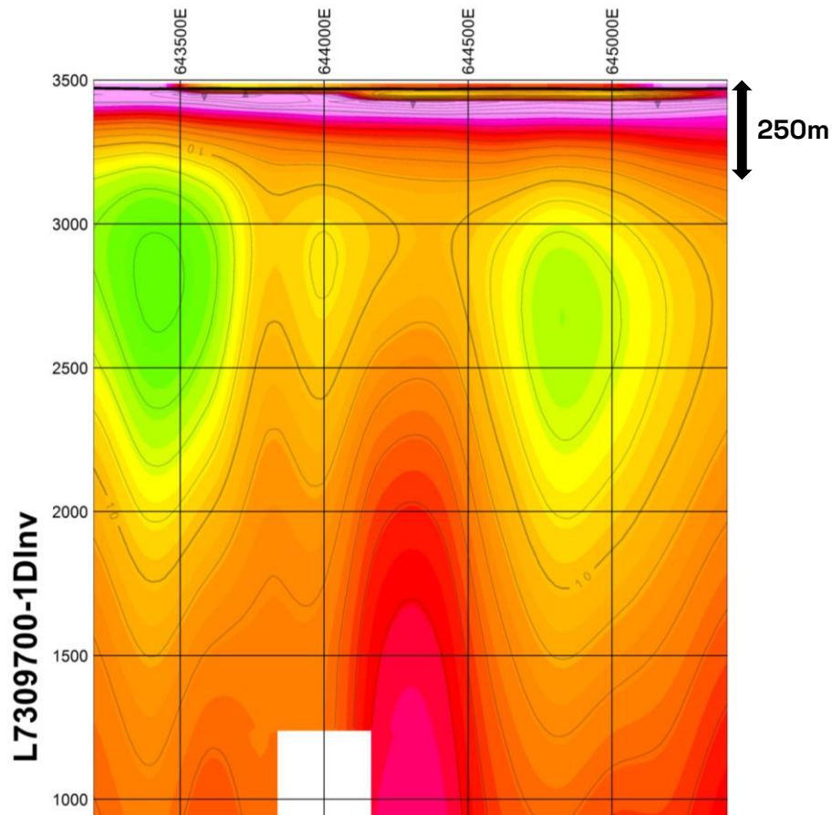
Candela II - Salar Incahuasi - MT Survey 1D & 2D Inversion Model Resistivity Sections
